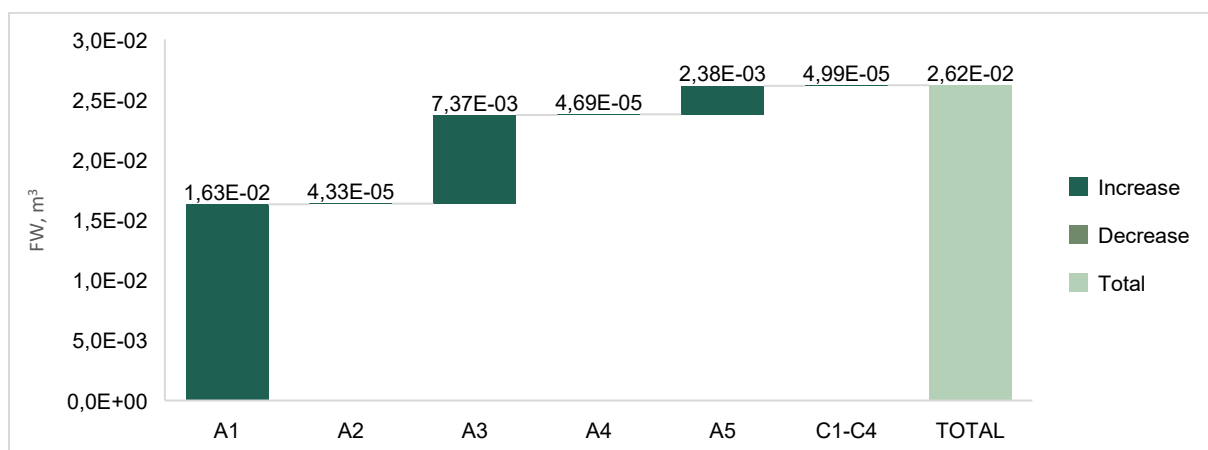
Net freshwater use for 1 m 2 of installed Knauf White 12.5mm gypsum plasterboard
