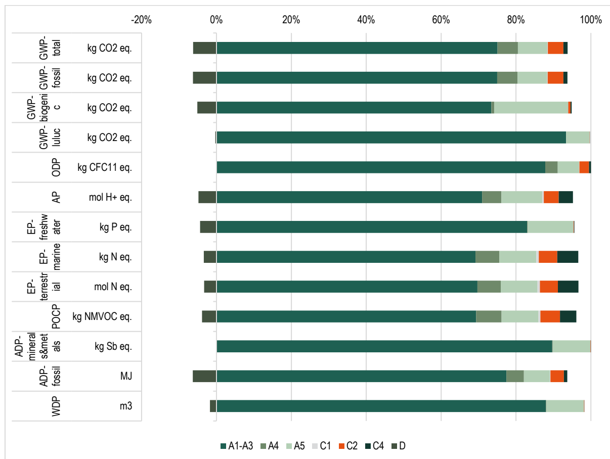
Contribution to environmental impact per each module for 1 m 2 of installed Knauf White 12.5mm gypsum plasterboard
