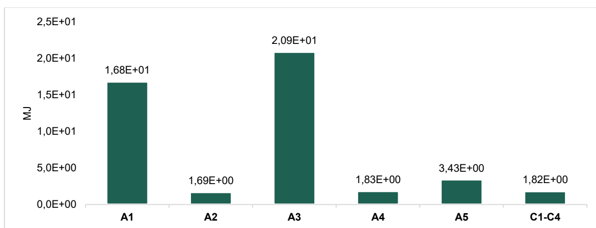
Primary energy demand per 1 m 2 of installed Knauf White 12.5mm gypsum plasterboard
